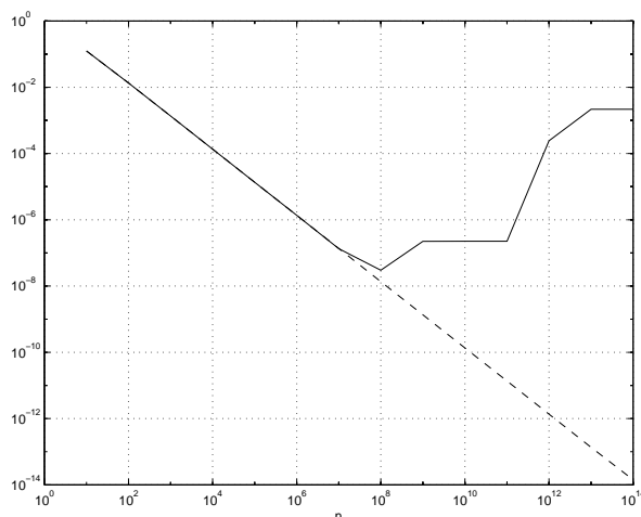
Figure 2.3.1. Computed values for n = 10^p , p = 1 : 14 , of the sequences: solid line |(1 + 1/n)^n - e| ; dashed line |\exp(n \log(1 + 1/n)) - e| using (2.3.4).
