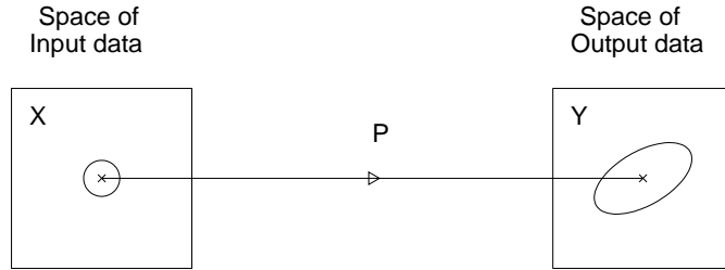
Figure 2.4.2. Geometrical illustration of the condition number.
